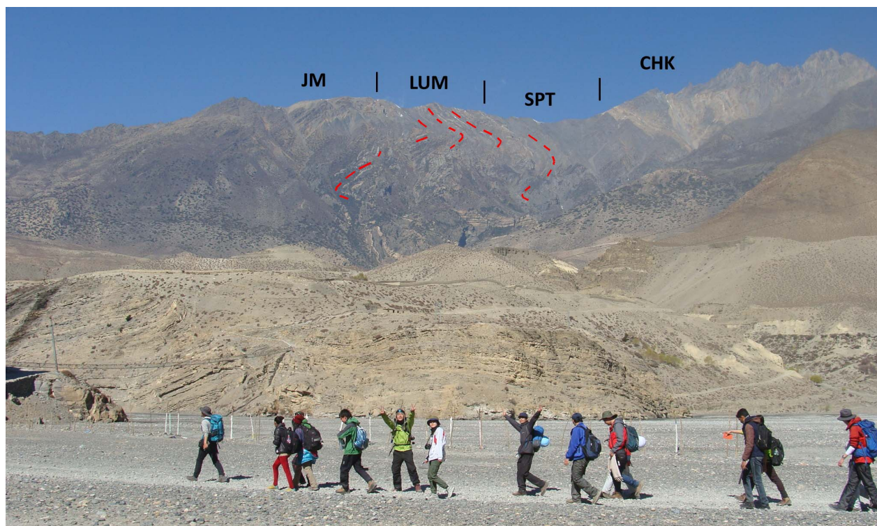
Walking on the wide Kaligandaki River with large foldings of Tethys formations on the back
